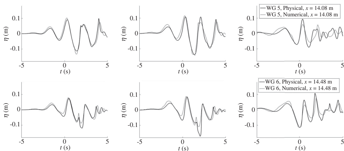
Figure 4 Predicted and measured free surface elevation time histories: left-hand column – group producing steep-fronted breaker; middle column – group producing plunging breaker; right-hand column – group producing broken wave
