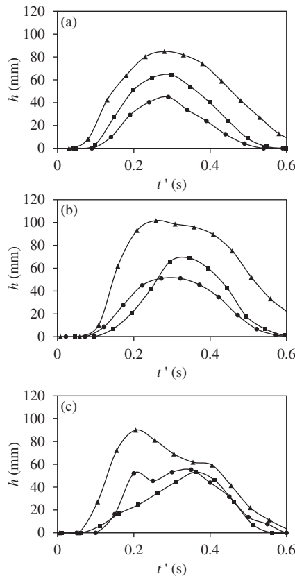
Figure 6 Overtopping flow layer thickness at seaward edge of the wall for (a) steep-fronted wave; (b) plunging wave; and (c) broken wave. ▲: 150 mm freeboard, ■: 200 mm freeboard, ●: 250 mm freeboard
