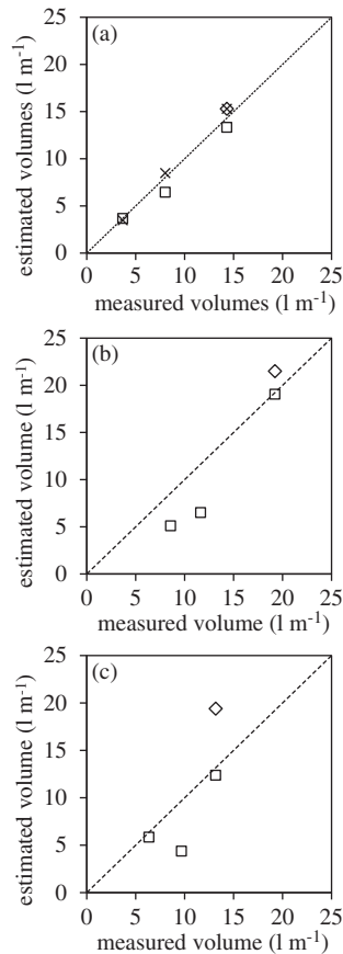
Figure 8 Estimated overtopping volumes compared with measured overtopping volumes for (a) steep-fronted wave; (b) plunging wave; and (c) already broken wave: \times , BIV; \diamond , numerical model; \square , weir analogy
